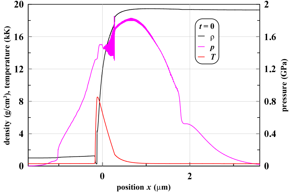
Figure 18. Profiles of density, temperature and pressure at time t = 0 . The pressure profile contains information about changes in the intensity of the laser pulse over time. The moment t = 0 is close to the moments of overturning of simple waves in water and gold: the steep sections on the pressure profile are close to the vertical segments at the points of inflection. By the time t = 0 , gold absorbed half the energy F_{\text{abs}}/2 of the incident pulse I(t) = I_0 \exp(-t^2/\tau_L^2) . In the calculation described in this paper, we have: \tau_L = 0.5 ns, F_{\text{abs}} = 900 mJ/cm 2 . At t > 0 , the intensity of I(t) decreases as compared with the maximum value of I_0 .
