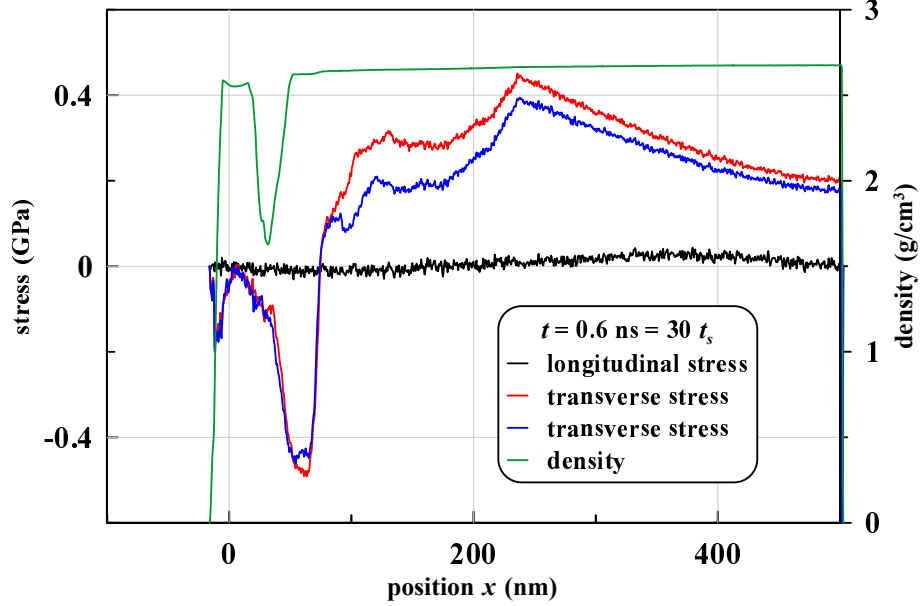
Figure 6. Final profiles are shown. They correspond to the late instant 0.6 ns. Density and symmetry maps for this time are presented in figure 3. We see creation of significant residual stress field. It relates to the residual deformations shown in figure 3. Here pressure components p_{ii} are shown. The stress components are \sigma_{ii} = -p_{ii} .
