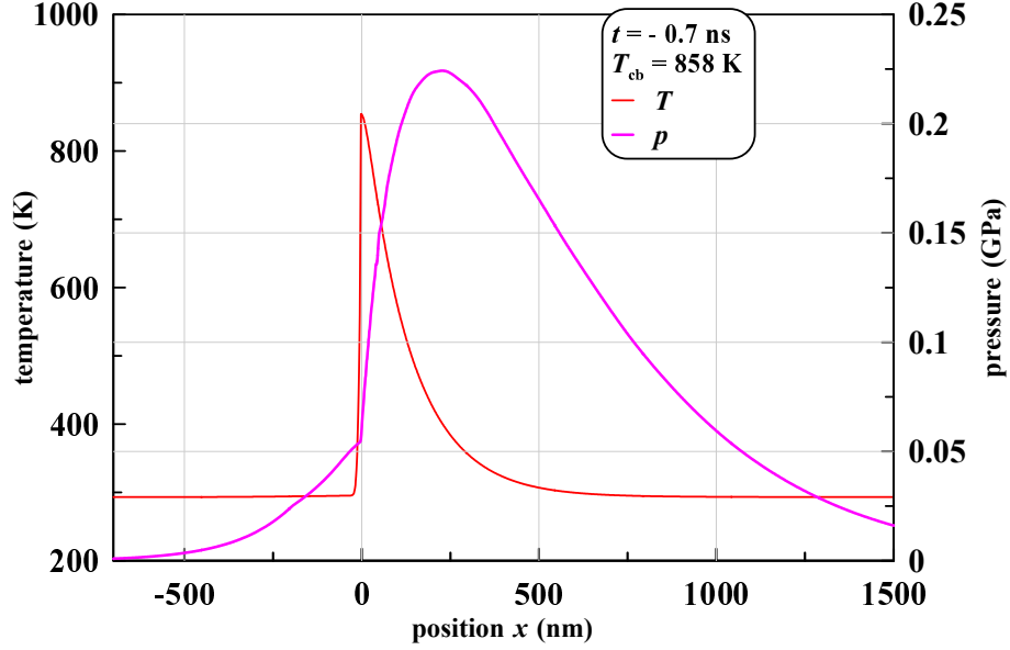
Figure 8. The situation at stage I, that is before melting, is shown. The calculation is started at t_{\text{ini}} = -1.5 ns. At this point, gold is to the right of the plane x = 0 , and water is to the left. The initial temperature of water and gold T_{\text{rt}} = 300 K. The heat spreads to gold at a depth of d_T = 0.1 \mu\text{m} . In the plane at a depth of d_T the temperature is (T_{\text{max}} - T_{\text{rt}})/2 + T_{\text{rt}} = (T_{\text{max}} + T_{\text{rt}})/2 , that is d_T = 0.1 \mu\text{m} is the full width at half-height by temperature increase. The pressure profile has smooth acoustic wings on the left and right.
