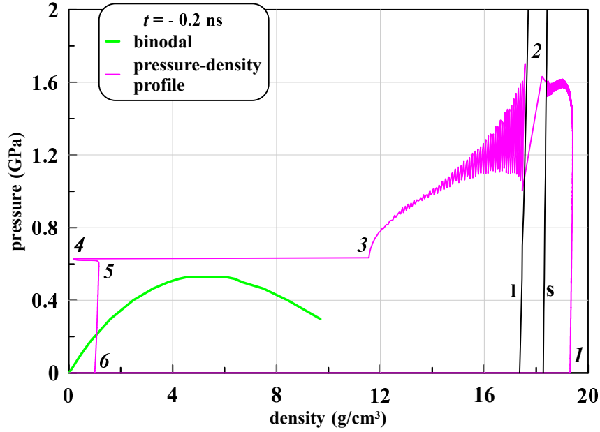
Figure 17. The hydrodynamic profile is built together with the phase equilibrium curves on the \rho, p . plane. Numbers 1–6 indicate the same states as in the previous figure 16. We see that the pressure at the hottest point of gold is still above the critical pressure of gold. The hottest is point 3. It is on contact with water. The letters s (solidus) and l (liquidus) indicate melting curves bordering the corridor of the existence of a mixture of solid and liquid phases. The intersection of this corridor with the instantaneous profile of the density and pressure distributions corresponds to segment 2 in figure 16. The pressure at the intersection of the melting front abruptly decreases, compare with pictures 13 and 14. This is caused by spatial expansion of liquid relative to solid crossing the melting front.
