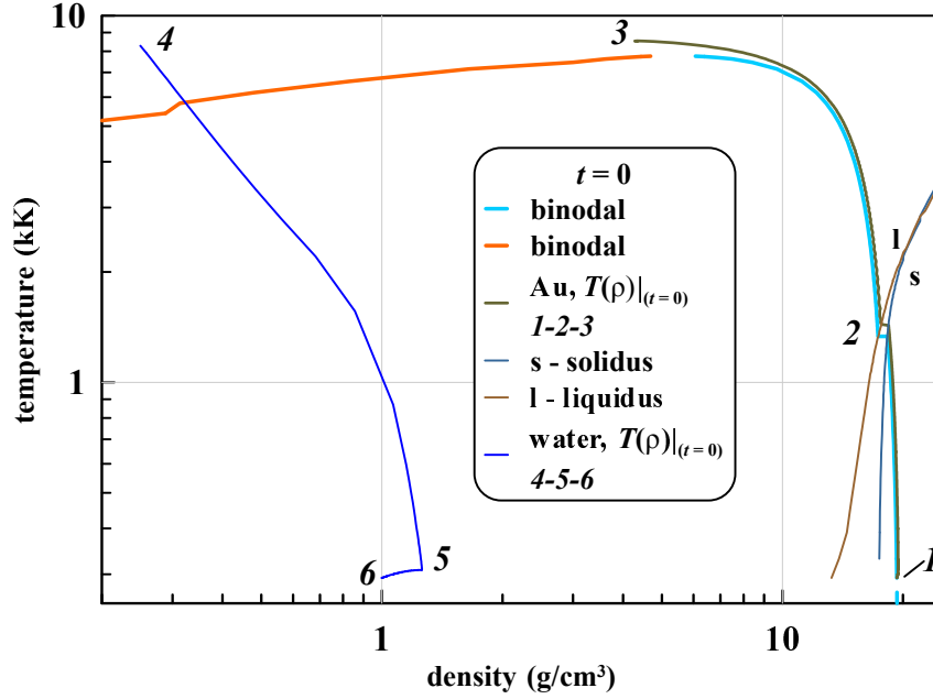
Figure 20. Temperature profile T(\rho, t)|_{(t=0)} on the phase plane \rho, T . The gradual heating by the laser leads to the fact that the temperature on the profile T(\rho, t)|_{(t=0)} rises above the critical value T_{cr} = 7.8 kK. The single (for water and Au) profile T(\rho, t)|_{(t=0)} is divided into two 1-2-3 (Au) and 4-5-6 (water) pieces. A density jump of 3-4 refers to the contact boundary, compare from figure 16, where a single profile is shown. Au and water densities at the contact are 4.35 and 0.25 g/cm 3 . A single density profile shows a profile where gold and water are not separated. Here they are separated. Curves s (solidus) and l (liquidus) are continued through the triple point to the metastable area [55–60]. Point 1 corresponds to gold at a great distance from the contact, where the temperature is equal to room temperature 300 K.
