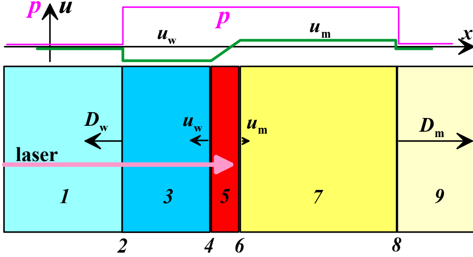
Figure 7. Figure illustrates laser heating of a metal target through water. Main ideas of the model developed in [49] are presented. The laser passes through unperturbed water 1, crosses the shock wave front 2, passes through the shock-compressed water 3 and is absorbed in the hot metal layer 5. The pulse is long in time (“subsonic” heating) in the sense that the sound scale L/c_s is much shorter than the pulse duration \tau_L , here L is the width of layer 5. Therefore, boundaries 4 and 6 of layer 5 act as two subsonic pistons pushing waves 2 and 8. Waves 2 and 8 propagate much faster than the expansion rate of layer 5. Therefore, layer 5 is thin compared with layers 3 and 7.
