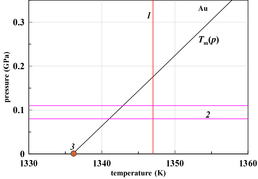
Figure 10. A small segment of the melting curve on the plane T, p is presented. This is the segment near the triple point marked with marker 3. A more complete phase diagram in the pressure range of interest is shown in the following figure 11. At the triple point, the melting point of gold (Au) is 1337 K. The lower and upper amplitudes of the tooth pressure, taken from figure 9, is shown here by two lines 2. Contact temperature T_{cb} = 1347 K in figure 9 is marked here by the vertical line 1. This temperature corresponds to the time t = -0.6 ns. As you can see, the temperature T_{cb} = 1347 K is 5 degrees higher than the melting point T_m|_{(p=943 \text{ bar})} = 1342 K. The pressure of 943 bar corresponds to the average pressure between the two horizontal lines 2.
