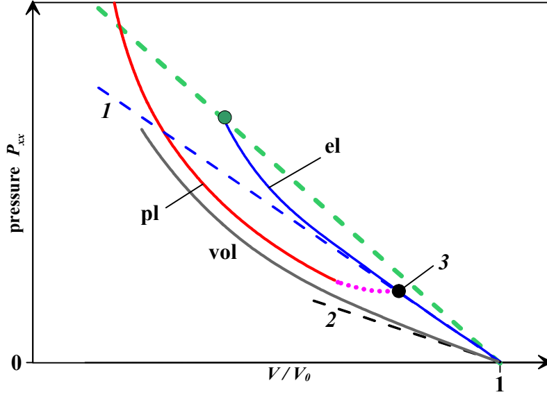
Figure 1. Comparison of hydrostatic (or volume, the curve “vol”) and uniaxial compressions. “Volume” means homogeneous shrink along all three spatial axes. There are two types of the uniaxial compressions. One is the elastic (“el”) while the second is plastic (“pl”) compression. The “el” and “pl” stress curves relates to the corresponding Hugoniot curves. Elastic body is more rigid thus its Hugoniot is steeper. Initial volume is V_0 . Speeds of elastic and plastic sounds are straights 1 and 2, respectively; approximation of isotropic elastic-plastic body is considered. Black circle 3 indicates the Hugoniot elastic limit. The dotted piece of the “pl” Hugoniot corresponds to decaying plastic shocks observed in [11,27,28]. Although formally these shocks cannot be placed on the p - V diagram because they are not stationary.
