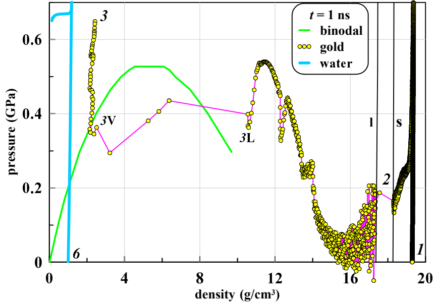
Figure 24. The plane \rho, p is important for the interpretation of mechanical phenomena. The compression wave in gold (see figure 22) is cut off here to increase the vertical scale. We clearly see appearance of gaseous gold 3-3V with s > s_{cr} . This layer of gold will condensed later into nanoparticles during expansion and cooling. Addition to nanoparticles from evaporation of the liquid gold 3L-2 is small.
