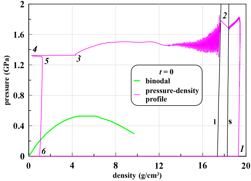
Figure 21. Pressure profile p(\rho, t)|_{(t=0)} on the phase plane \rho, p is shown. For the time elapsed from the previous time point t = -0.2 ns, see figure 17, the pressure has increased significantly: twice times near contact and 7% in its maximum value. The maximum pressure is in the solid phase behind the melting front—we have to average over oscillations in liquid. The meaning of numbers 1–6 is the same as in figures 16, 17 and 20. Note that the corresponding to gold 1–2–3 profile, which was just above the boiling curve in figure 20 and 16, here it is far removed from the boiling curve. This is due to the low compressibility of the condensed phase. Surprisingly, this is also true for states that are to the left of a critical point on the density axis.
