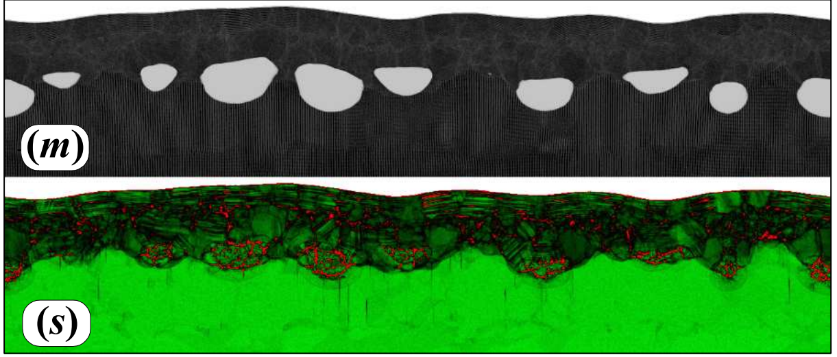
Figure 3. Frozen nano-structures remaining in a thin subsurface layer after action of a picosecond laser pulse are shown. The upper panel ( m ) gives density distribution. The bottom panel ( S ) demonstrates distribution of a symmetry factor S . The factor shows local order of a crystalline lattice. Green colors correspond to a solid state. Regions colored with deep green shows nano-crystalline aluminum. We are interested in the residual deformations produced in a target by an ultrashort laser pulse. From this point of view, melting, nucleation and freezing of nano-cavities is a side effect. The horizontal dimension is 0.5 micron.
